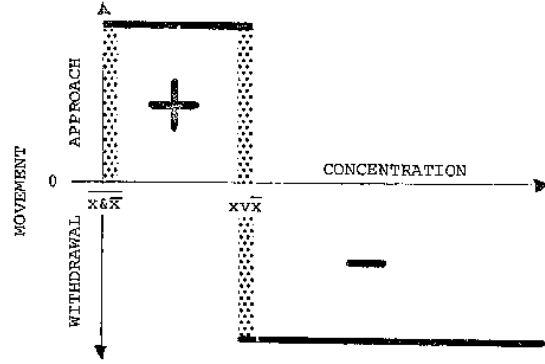
Fig. 2. The laws of “excluded contradiction” ( \overline{x \& x} ) and of “excluded middle” ( x \vee \overline{x} ) in the twilight zones between no motion ( M = 0 ) and approach (+), and between approach (+) and withdrawal (-) as a function of the concentration ( C ) of a perceptible agent.
